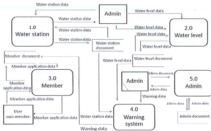
Figure 2 Data flow diagram (DFD)
