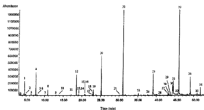
Fig. 1 GC-MS TIC profile of the aromatic volatile oil from fresh flowers of M. hortensis . See GC-MS analysis condition and Table I for peak identifications.
