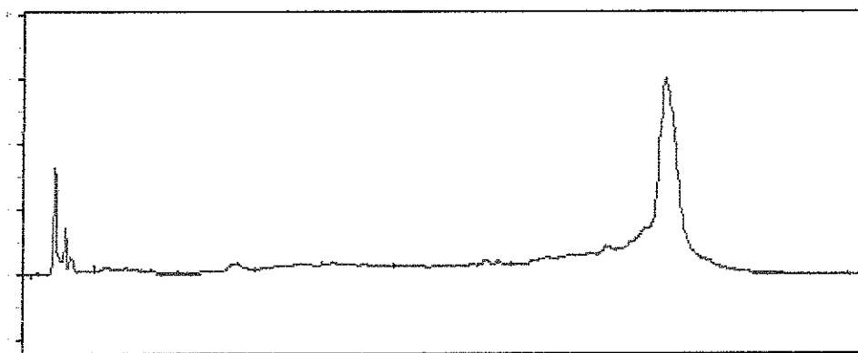
Figure 5: Chromatograms of sample using Ultra C18 column, 5 \mu m, 150x4.6 mm after load with Non-MIP column
