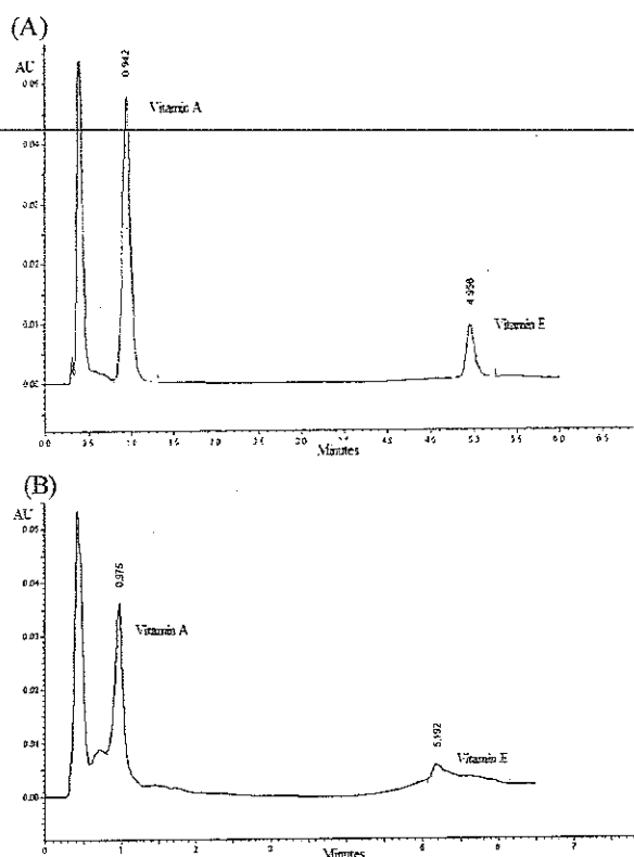
Figure 2 (A) Chromatogram of a standard mixture of vitamin A (retinol) and vitamin E ( \alpha -tocopherol), each at a concentration of 10 \text{ mg L}^{-1} ; (B) chromatogram of an avocado nanoemulsion lotion sample (Booth 7)
