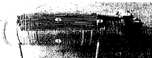
Figure 1. Lab-scale ginger washer/peeler: 1) motor, 2) water tank, 3) rolling vessel and 4) stainless steel grates
